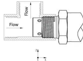
Figure 4. Installation Method (3)
