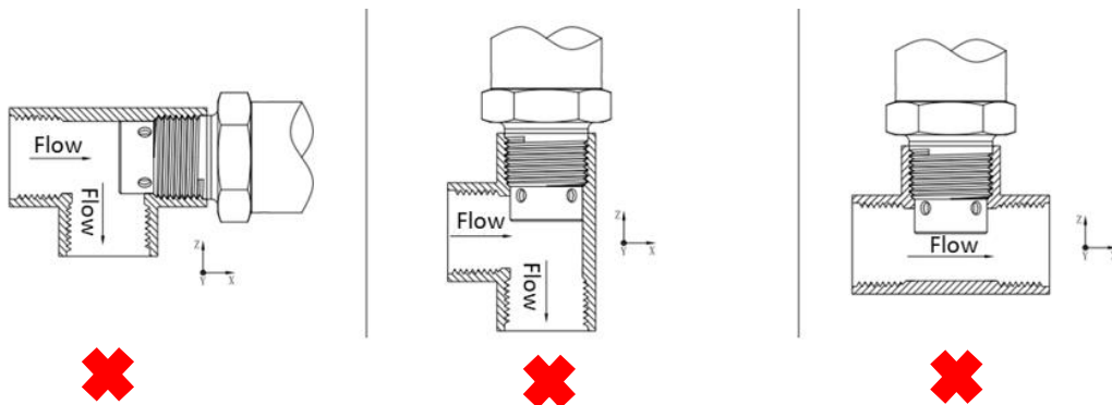
Figure 5. Installation methods to be avoided .
