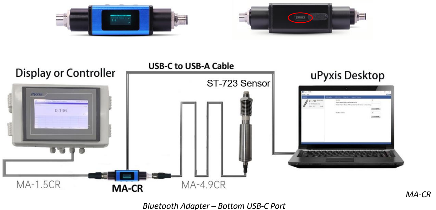
Figure 13. ST-723 Probe / MA-CR / USB-C Cable connected to uPyxis Desktop.
