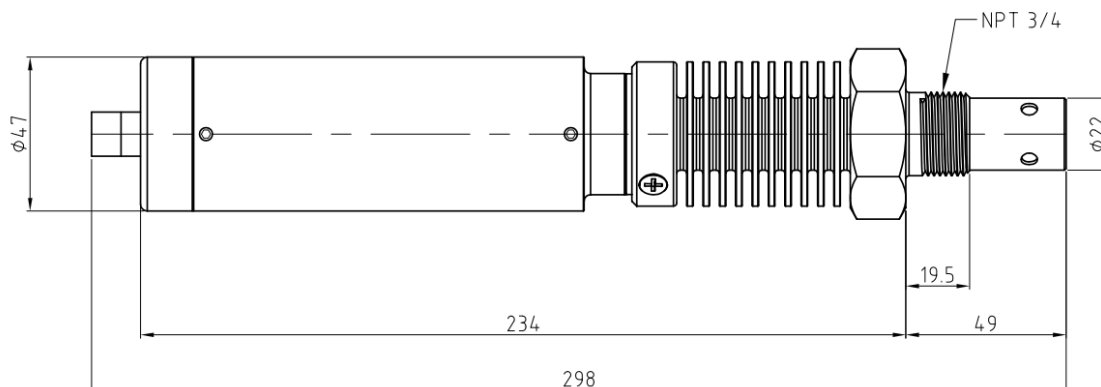
Figure 1. Dimension of the ST-723 (mm)
