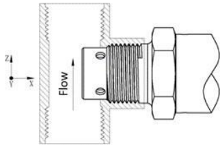
Figure 2. Installation Method (1)
